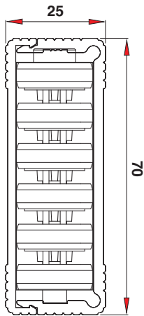
40A 6mm x 3mm CUPONAL™ Bar's
