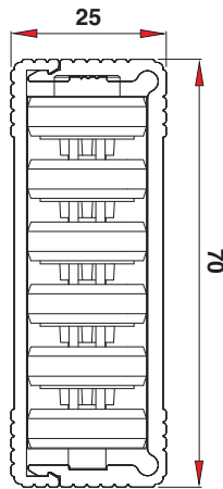
63A 8mm x 3mm CUPONAL™ Bar's
